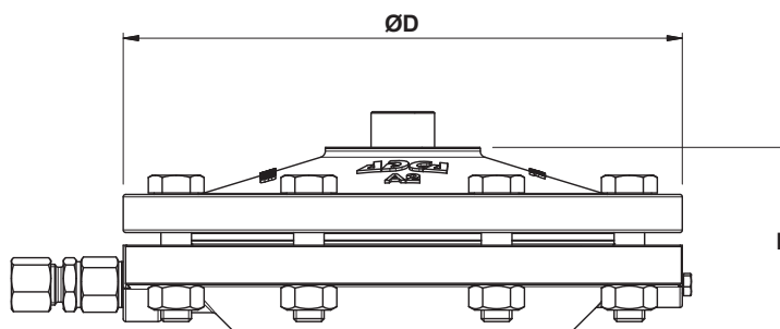
DIMENSIONS – ACTUATOR (mm)
